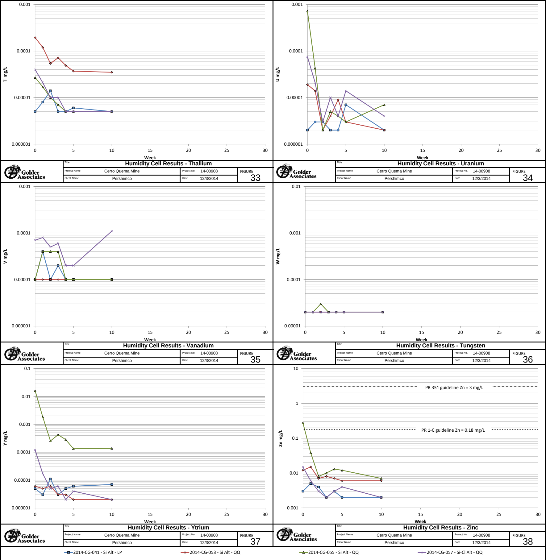
Figure C-1 Kinetic Testing Results Cerro Quema Project
