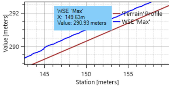
Water Surface Elevation on 'Profile 1'
