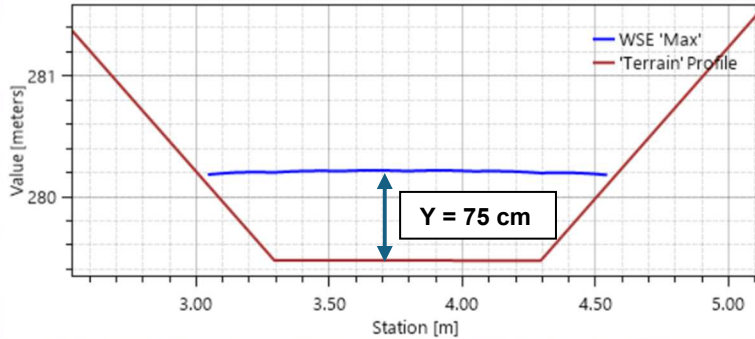
Water Surface Elevation on 'CAJON02'
