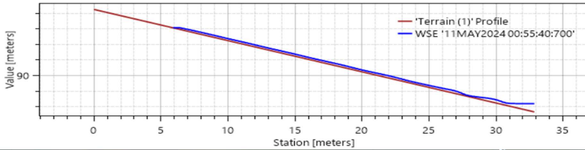
Water Surface Elevation on 'Profile 1'
