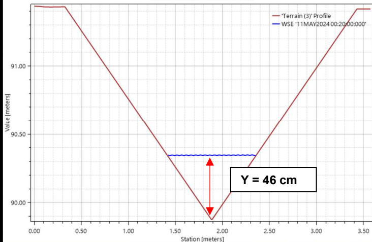
Water Surface Elevation on 'CAJON'
