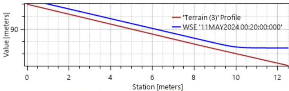
Water Surface Elevation on 'CAJON'
